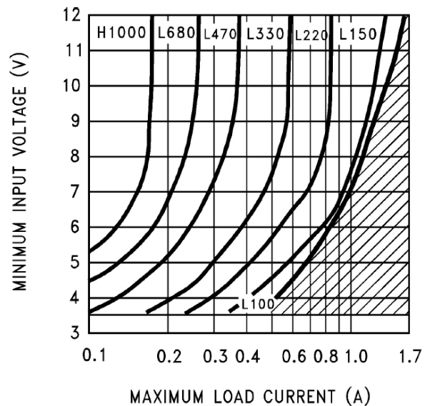
FIGURE 8. LM2577S/T_ADJ-15
