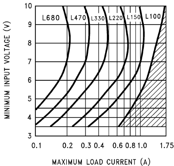
FIGURE 7. LM2577S/T_ADJ-12 Inductor Selection Guide
