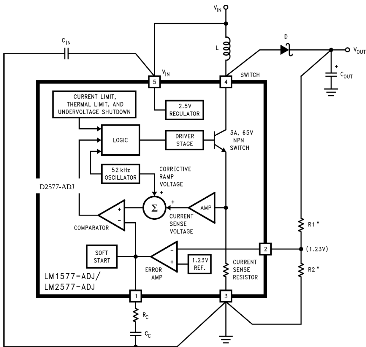
FIGURE 4. LM2577S/T_ADJ Block Diagram and Boost Regulator Application
